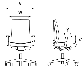
NAVIGO UPH FS R35K2 TS25 (ST44) ESH Weight | Poids: 16.25 kg (16.50 kg) NAVIGO MESH/MESH PLUS Weight | Poids: 15.75 kg (16.00 kg)
