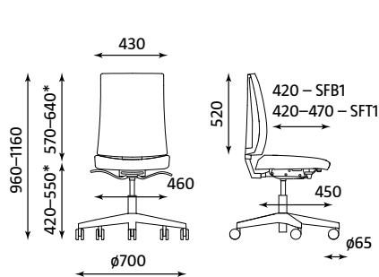
NAVIGO UPH SFB1 RTS TS25 (ST44) ESH Weight | Poids: 14.80 kg (15.05 kg) NAVIGO MESH/MESH PLUS Weight | Poids: 14.30 kg (14.55 kg)
