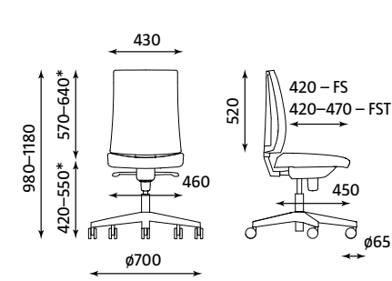
NAVIGO UPH FS RTS TS25 (ST44) ESH Weight | Poids: 14.65 kg (14.90 kg) NAVIGO MESH/MESH PLUS Weight | Poids: 14.15 kg (14.40 kg)
