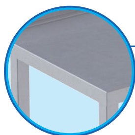
10 mm groove preventing water from dripping
